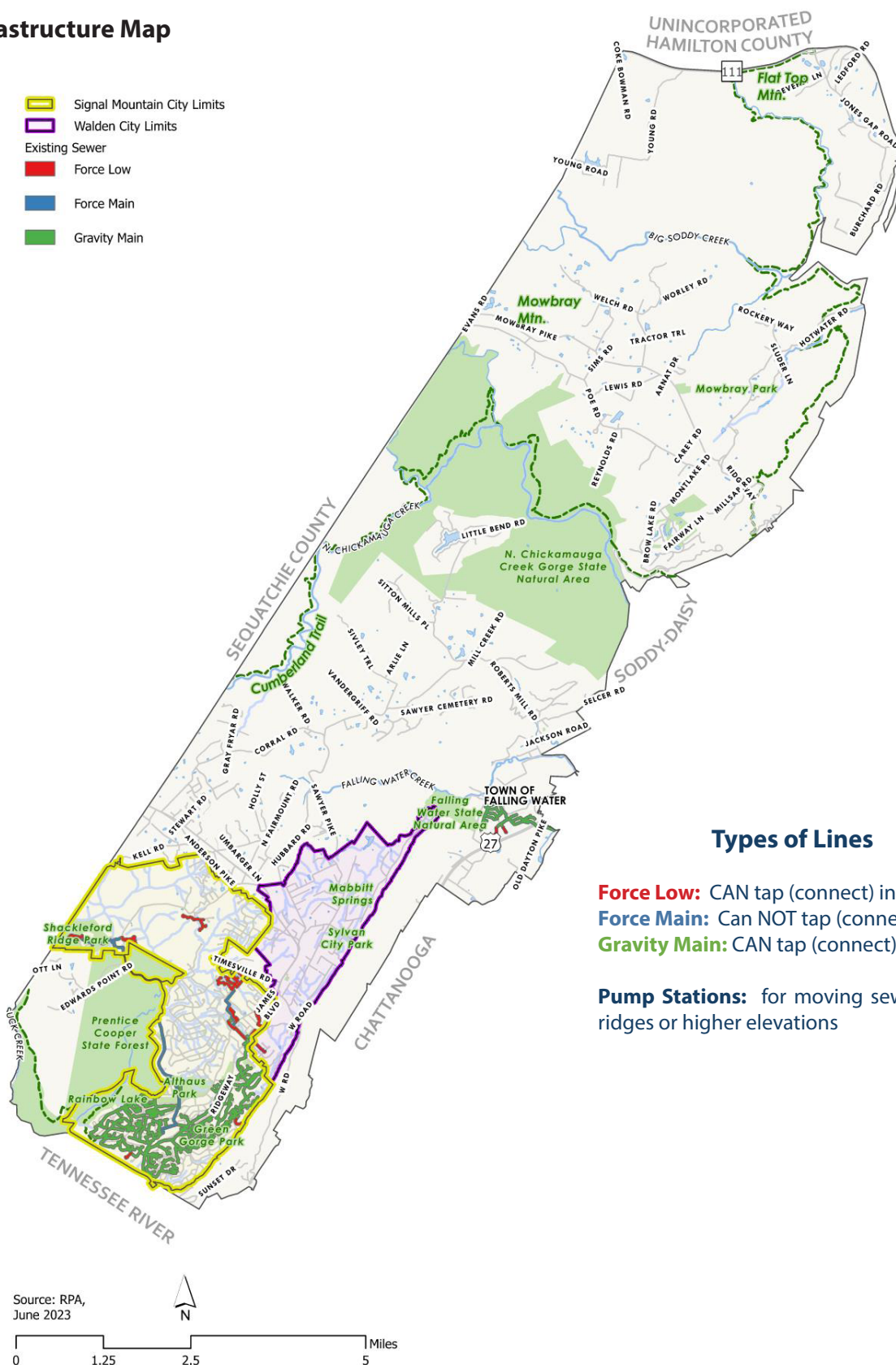
Figure 2.5: Sewer Infrastructure Map
